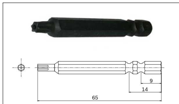
6-Lobe LONG BIT for TRF®
