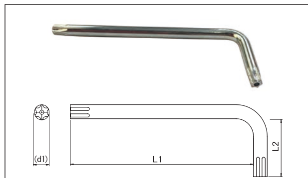
6-Lobe KEY for TRF®
