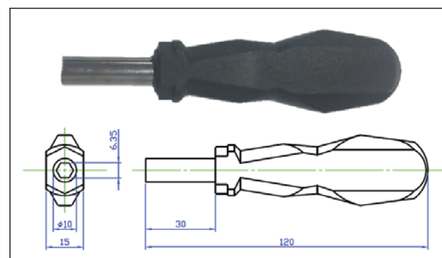
BIT HOLDER
