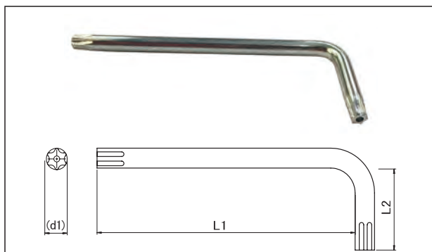
6-Lobe KEY for TRF®
