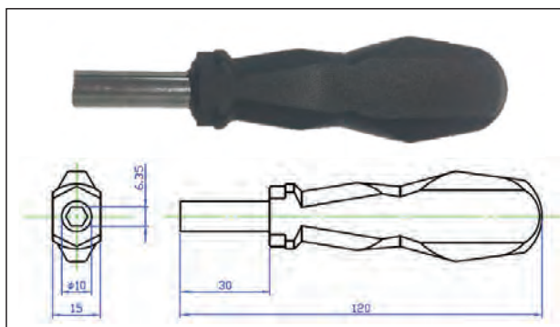
BIT HOLDER
