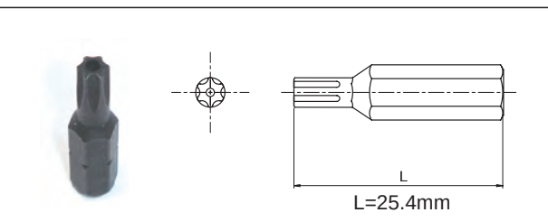
6-Lobe BIT for TRF®
